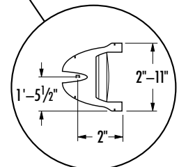
Location of "stub" for water supply at base of ladder
